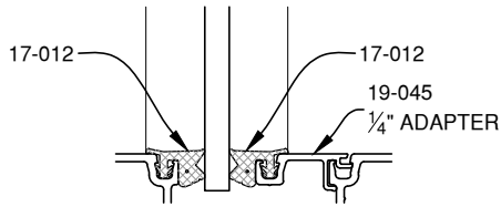
1/4" GLAZING
