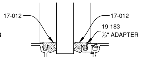
5/8" GLAZING
