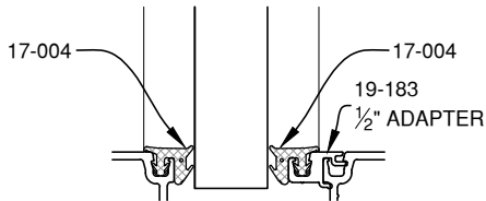
3/4" GLAZING
