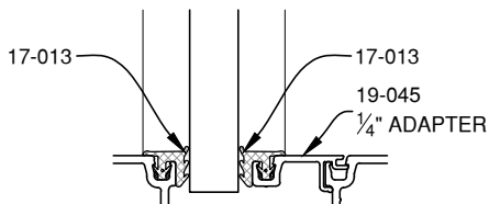
1/2" GLAZING
