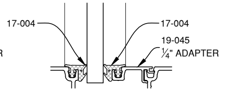
3/8" GLAZING
