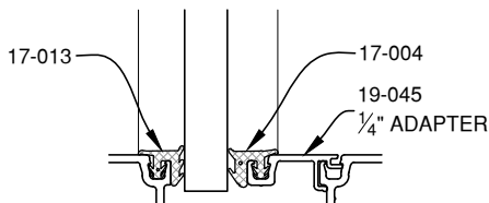
7/16" GLAZING
