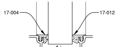
1 1/16" GLAZING
