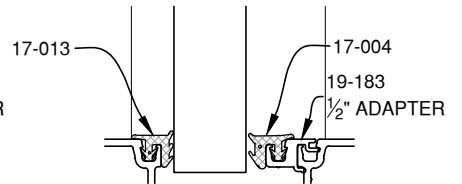
13/16" GLAZING
