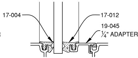
5/16" GLAZING
