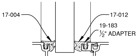
11/16" GLAZING
