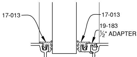
7/8" GLAZING
