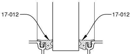
1" GLAZING
