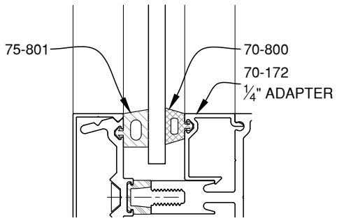
1/4" GLAZING
