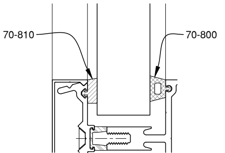
1 1/8" GLAZING
