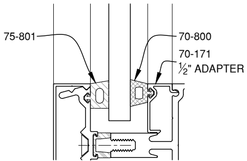
7/16" GLAZING
