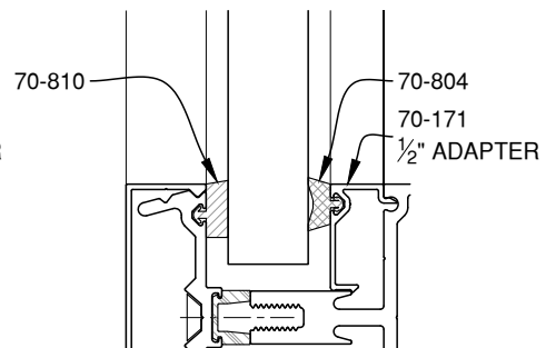
3/4" GLAZING
