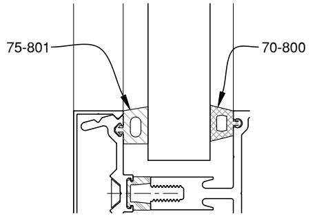
15/16" GLAZING
