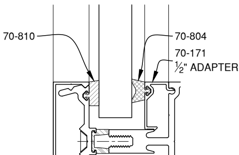
11/16" GLAZING
