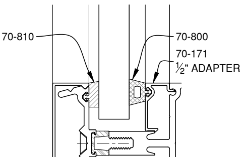
5/8" GLAZING
