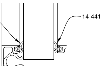
1 1/16" GLAZING
