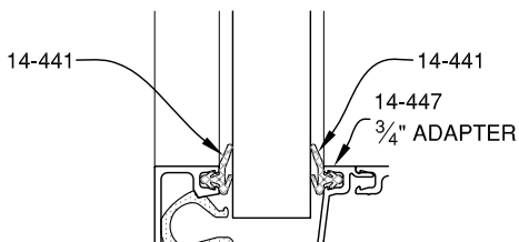
3/4" GLAZING
