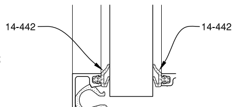
15/16" GLAZING
