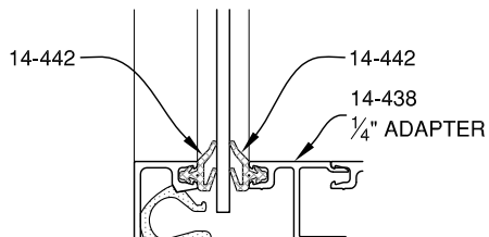
1/8" GLAZING
