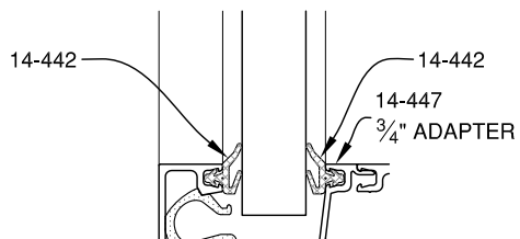
5/8" GLAZING
